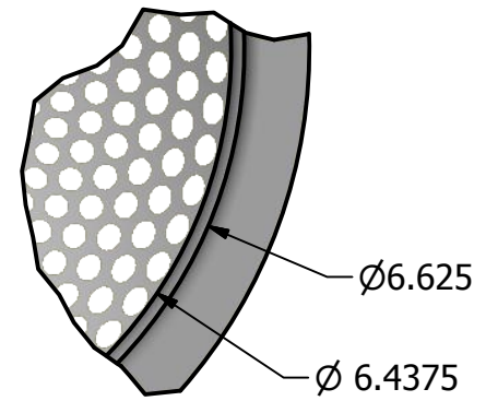
DETAIL B SCALE 2 / 3
