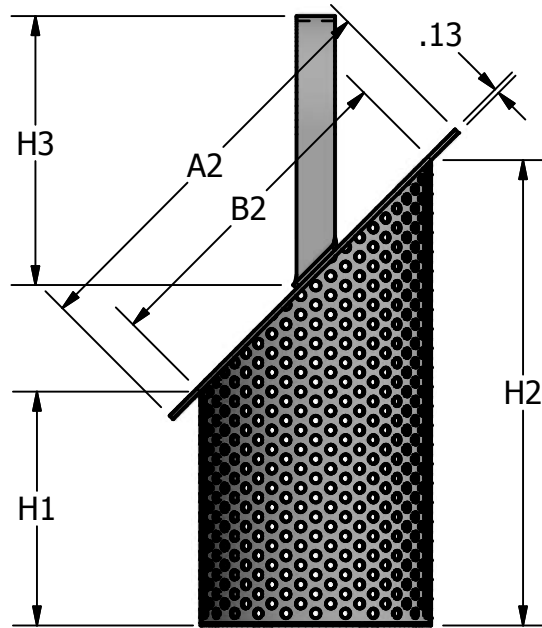
VIEW B-B
